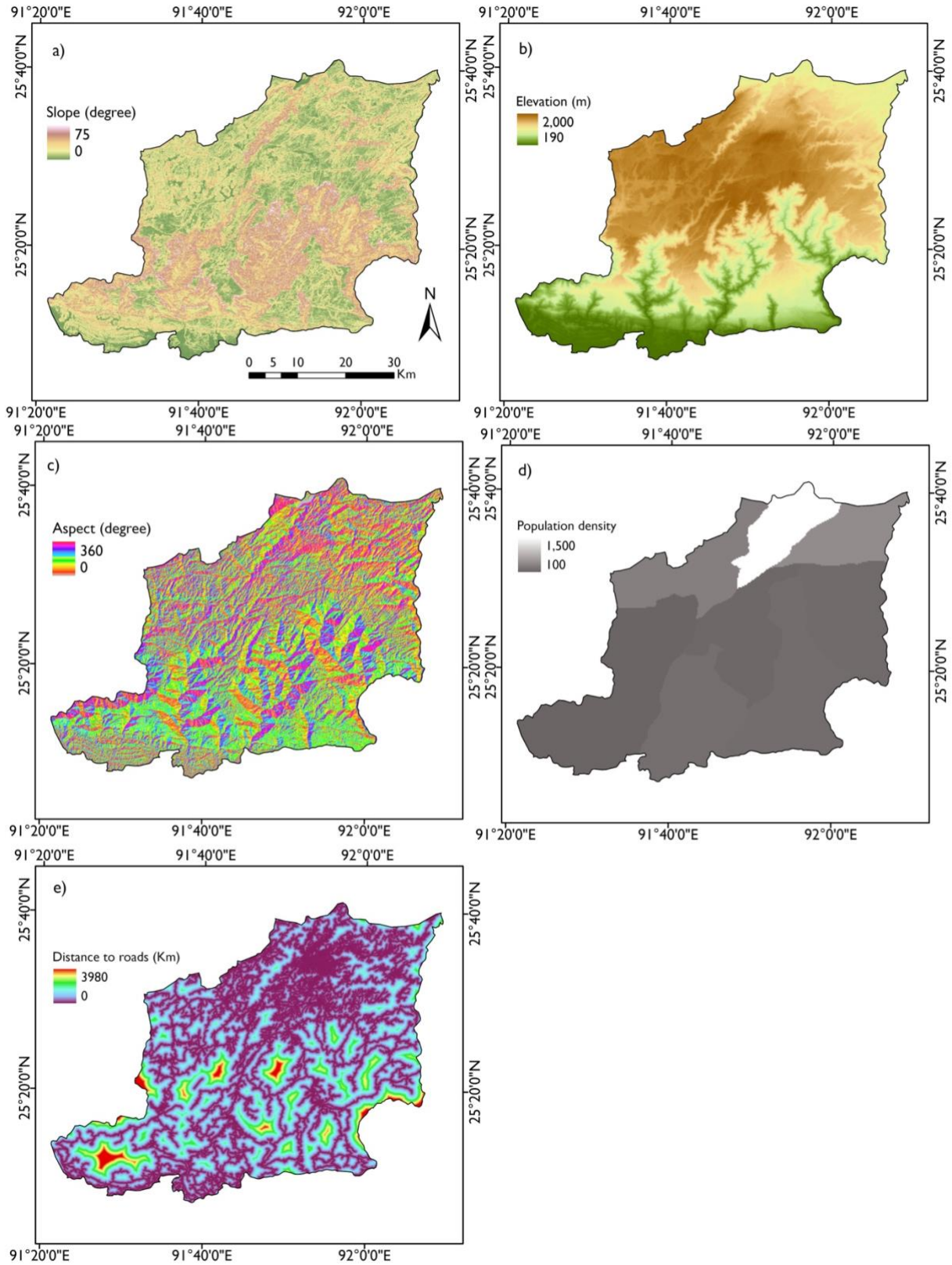
Figure 2. Spatial distribution of explanatory variables: a) Slope, b) Elevation, c) Aspect, d) Population density, and e) Distance to roads.
