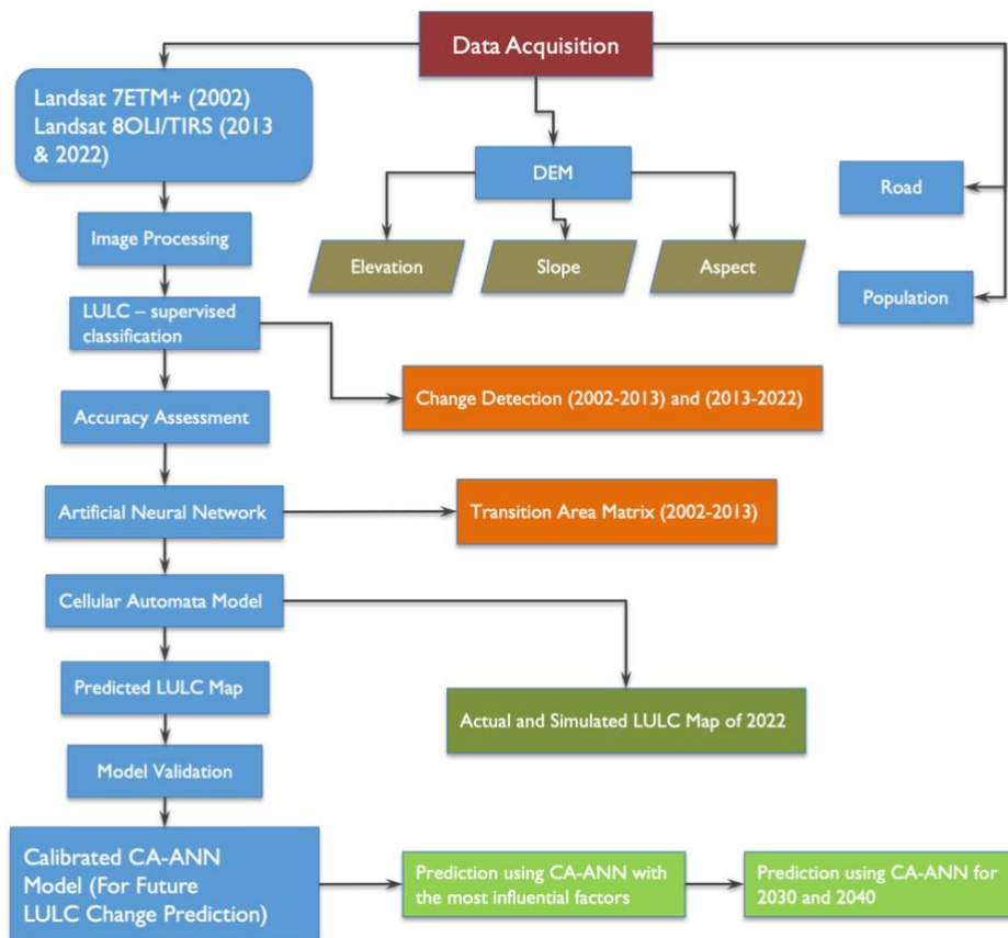
Figure 3. Flowchart showing the step-by-step analysis of Land Use and Land Cover (LULC) and their prediction using Cellular Automata–Artificial Neural Network (CA-ANN).
