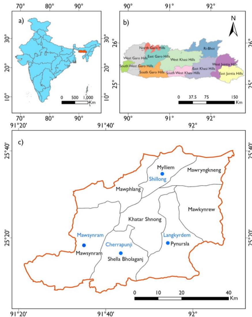
Figure 1. Map of the study area showing a) the state of Meghalaya in India (highlighted in red), b) the district boundary of the state of Meghalaya, and c) East Khasi Hills district including eight community and rural development blocks.
