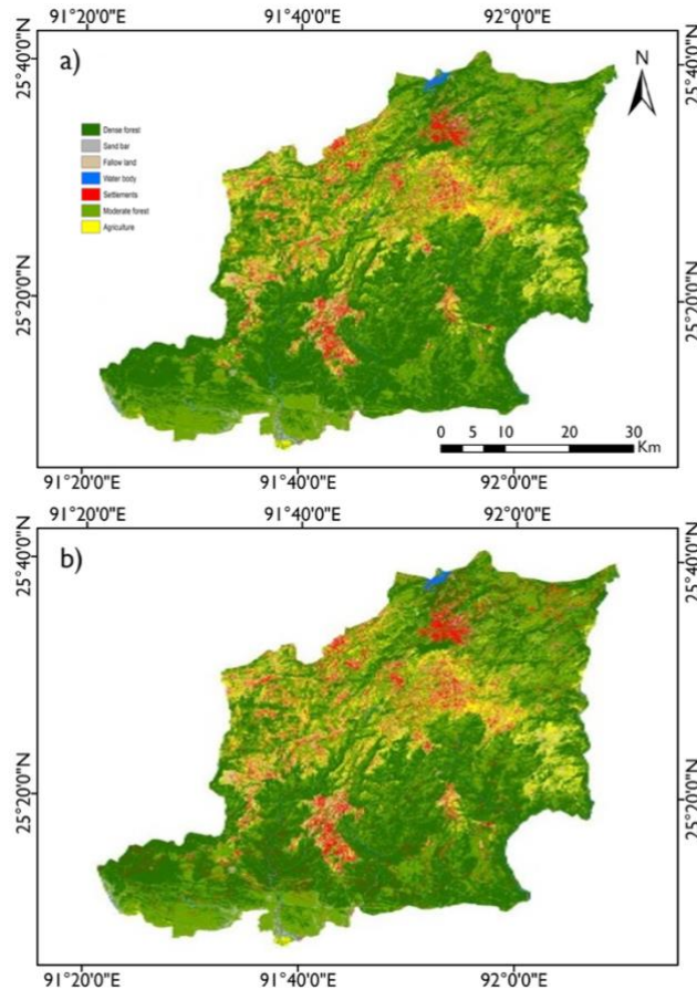
Figure 6. Predicted land use and land cover maps for the years: a) 2030, and b) 2040.
