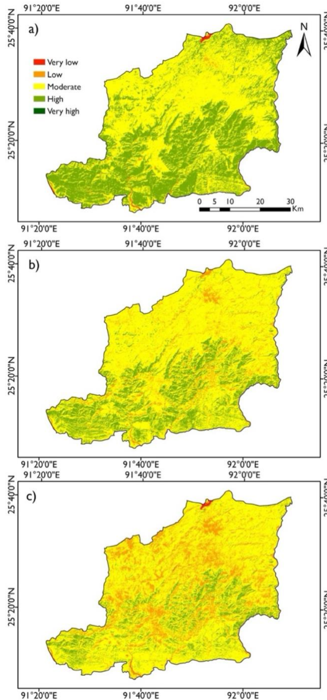
Figure 4. Comparison of NDVI values in East Khasi Hills district, Meghalaya, India, for the years: a) 2002, b) 2013, and c) 2022.
