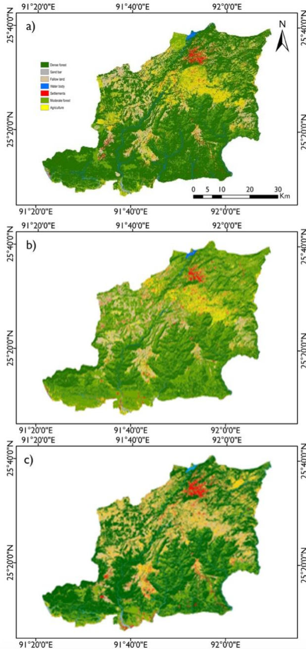
Figure 5. Land use and land cover maps for the years: a) 2002, b) 2013, and c) 2022.
