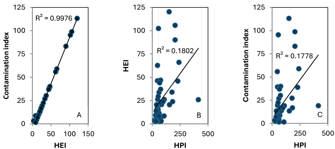
Figure S1. Scatter plot showing the relationship between a) HEI and contamination index ( C_d ), b) HPI and HEI, and c) HPI and contamination index ( C_d ).
