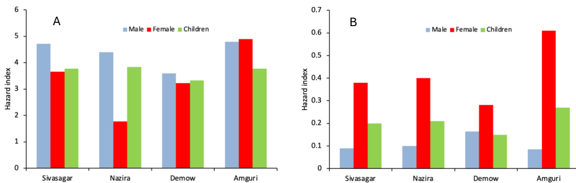
Figure S2. Non-carcinogenic hazard index (HI) through a) oral, and b) dermal exposure route in children, males and females.
